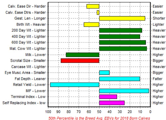
EBV Percentiles for NETHERTON MACHAU T885
